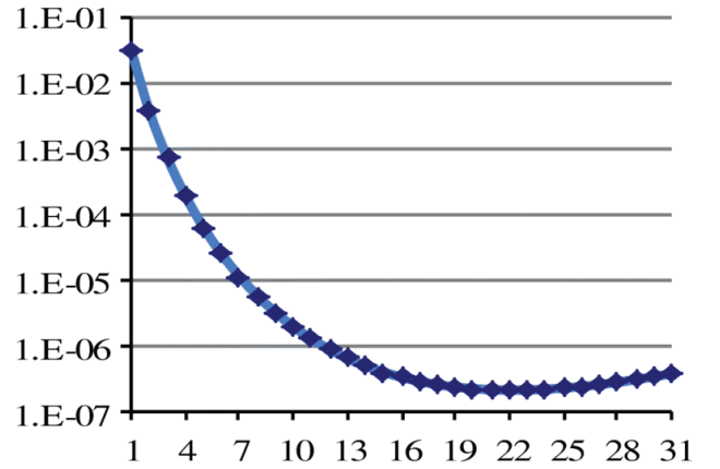
Fig. 4. Computation of false positive rate
